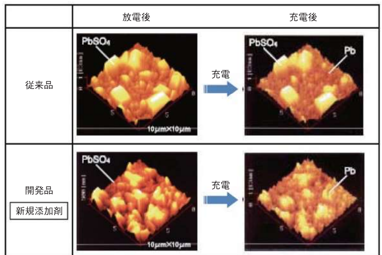
図4 AFMを用いた電極活物質の充放電中の形状変化のその場観察例 Figure 4 Images of in-situ AFM observations which visualize the morphology changes of electrode active materials during charge-discharge cycles
